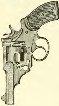
The Webley "Mark III.
